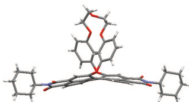
Figure 2. Molecular structure of racemic PBI 2a , as observed by single-crystal X-ray analysis. ( P )-enantiomer is depicted, view along the short axis of the PBI showing the bowl-like distortion of the perylene core.
