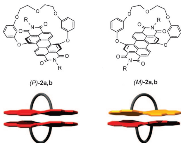
Figure 1. Structures of atropo -enantiomeric ( P )- 2a,b and ( M )- 2a,b and schematic representation of homo- and heterochiral dimer aggregates derived thereof.
